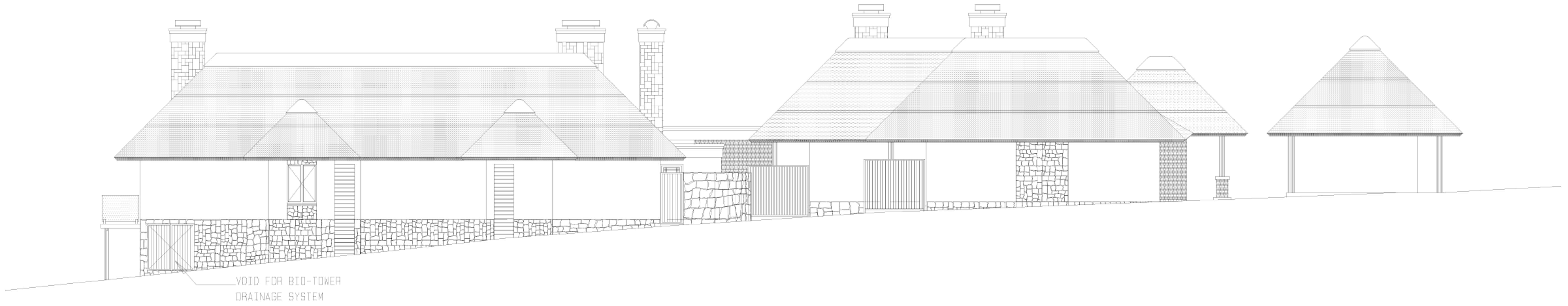
WEST ELEVATION
