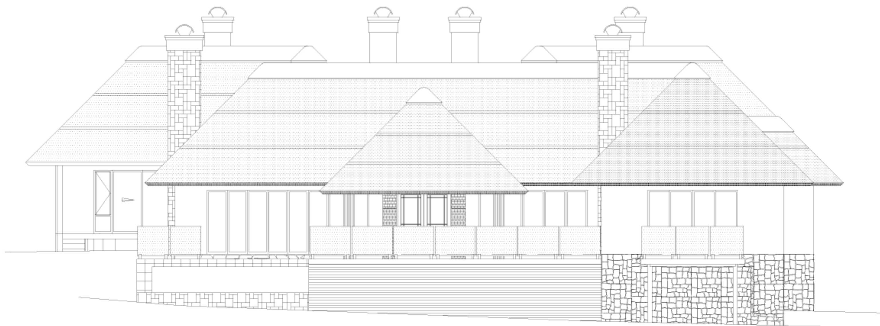
NORTH ELEVATION
